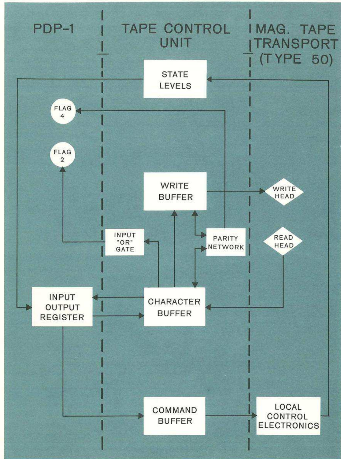
Magnetic Tape Control Block Diagram
