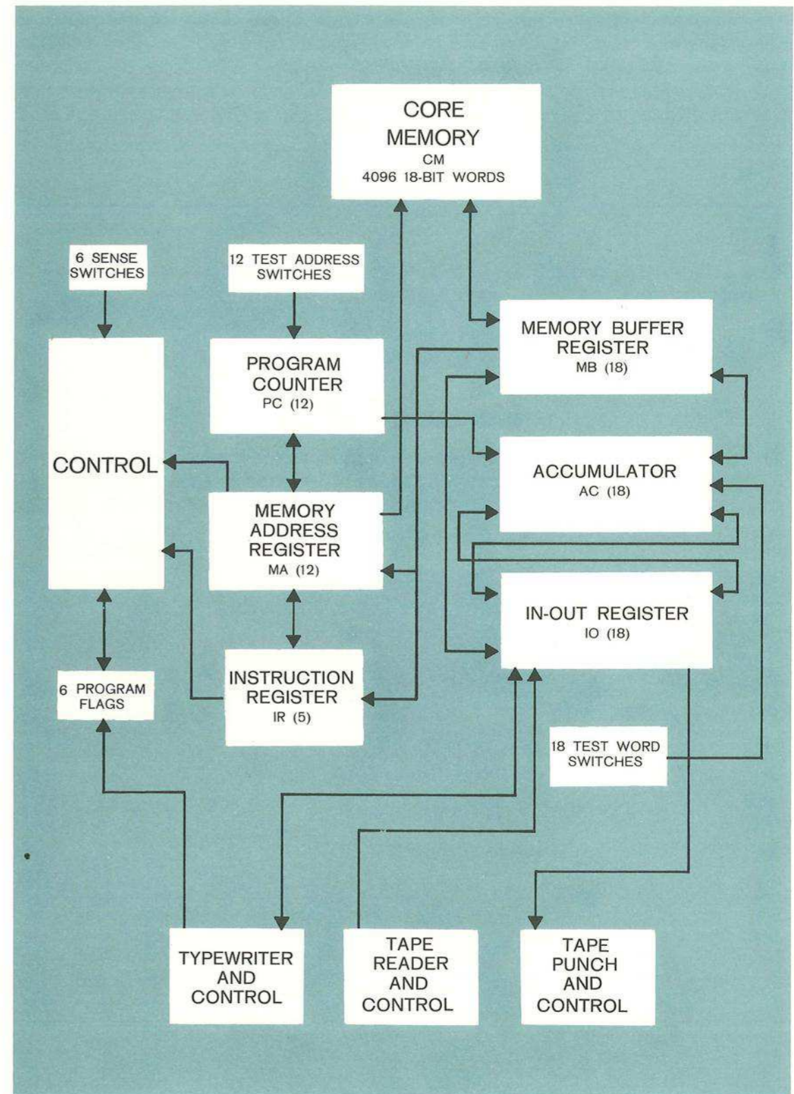
PDP-1 Logic Organization
