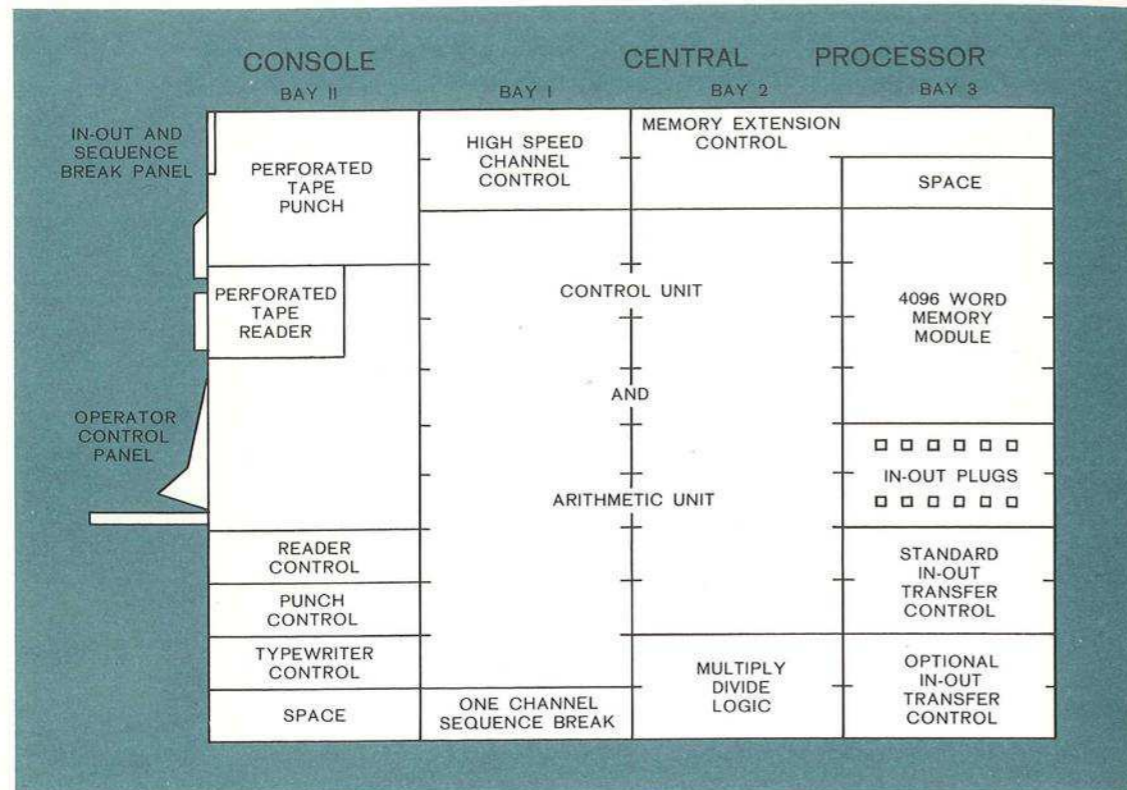
Central Processor Logic Layout, Side View
