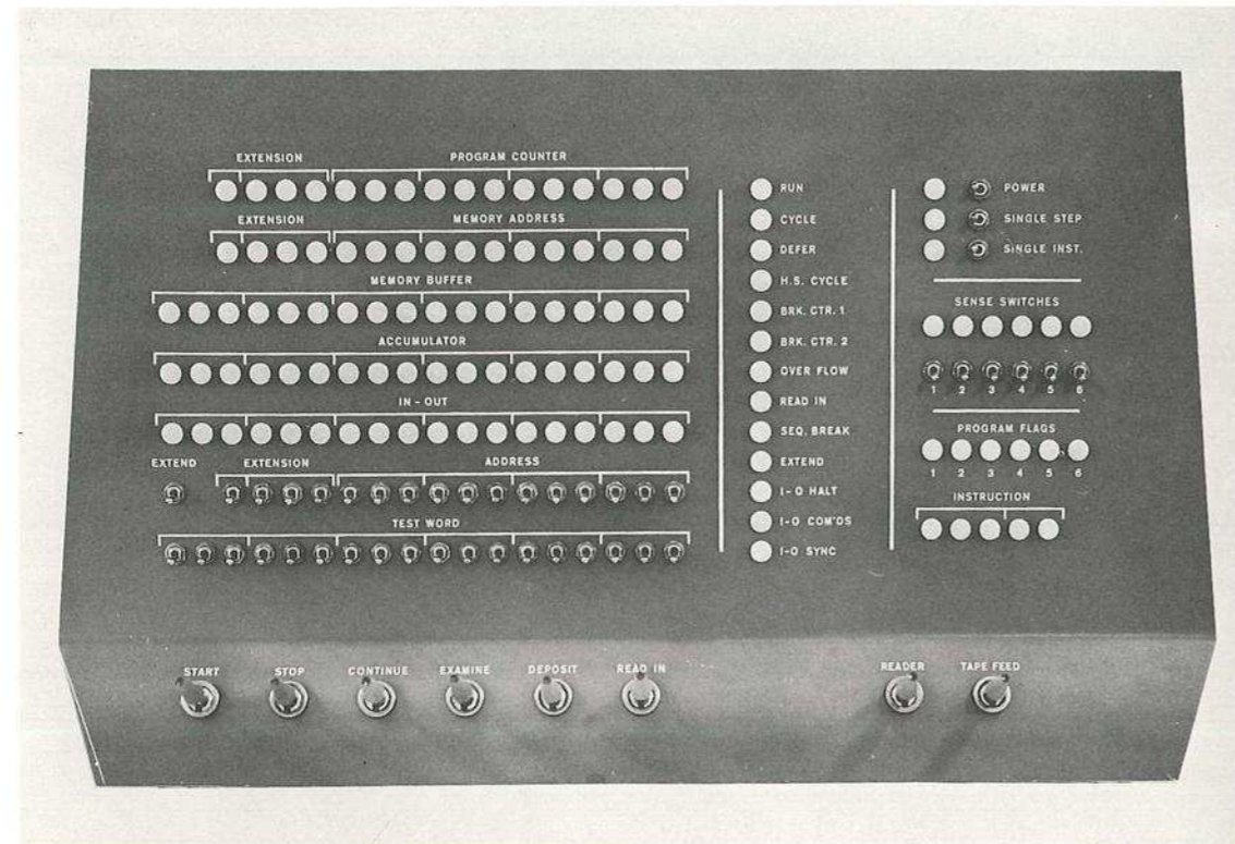
PDP-1 Control Panel
