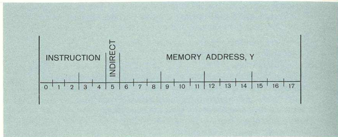
PDP-1 Instruction Format
