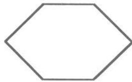
convex polygon
