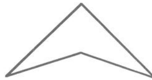
concave polygon
