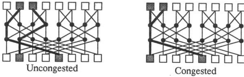
A 3-layer Omega Network
