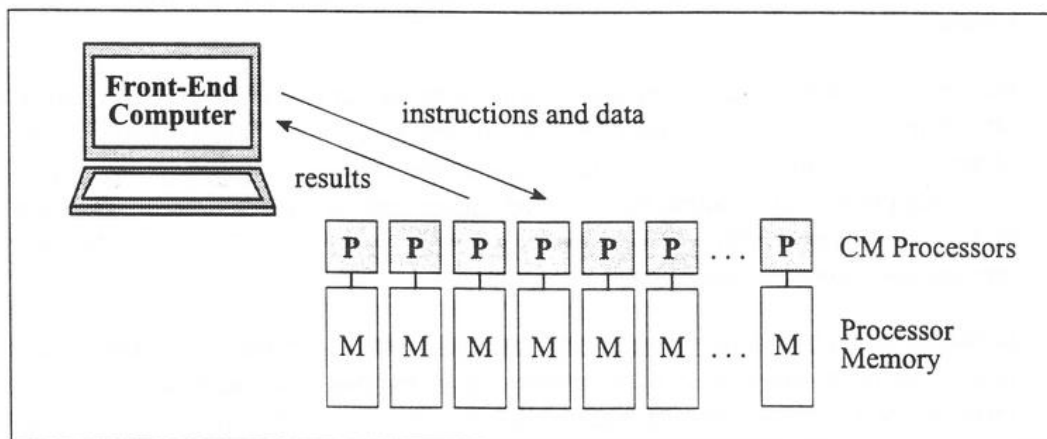
Figure 10. The data parallel programming model of the CM
